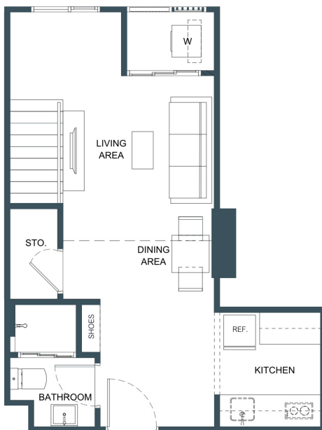
MAIN LEVEL
